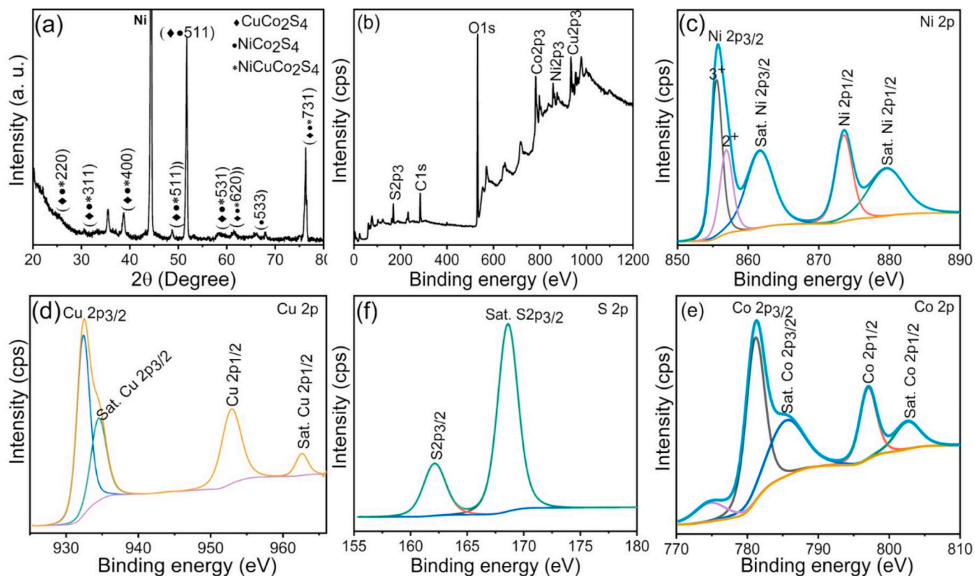
Fig. 3. (a) XRD pattern, (b) XPS survey spectra, (c) core levels of Ni 2p, (d) core levels of Cu 2p, (e) core levels of Co 2p, and (f) core levels of S 2p for the optimized \text{NiCuCo}_2\text{S}_4 .
